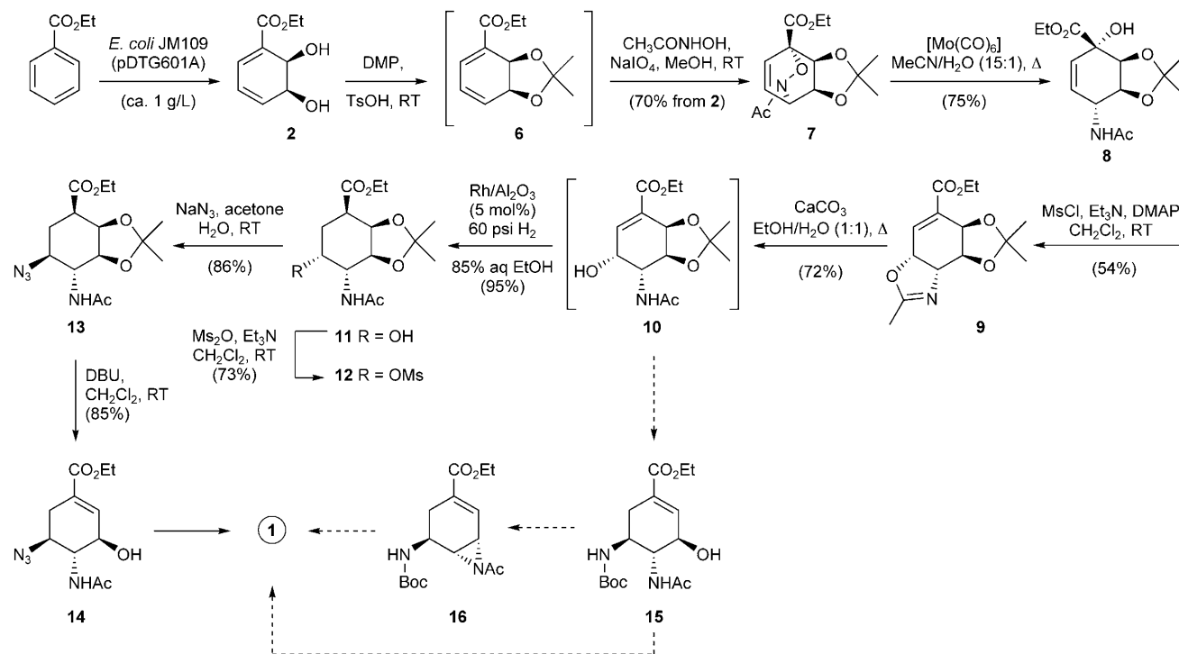
Scheme 2. Synthesis. DMP = dimethoxypropane, Ts = 4-tolylsulfonfyl, Ms = methanesulfonyl, DMAP = 4-dimethylamino pyridine, DBU = 1,8-diazabicyclo[5.4.0]undec-7-ene.
